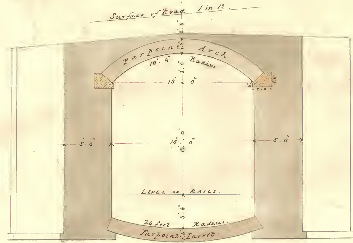
SQUARE SECTION THROUGH ARCH.
