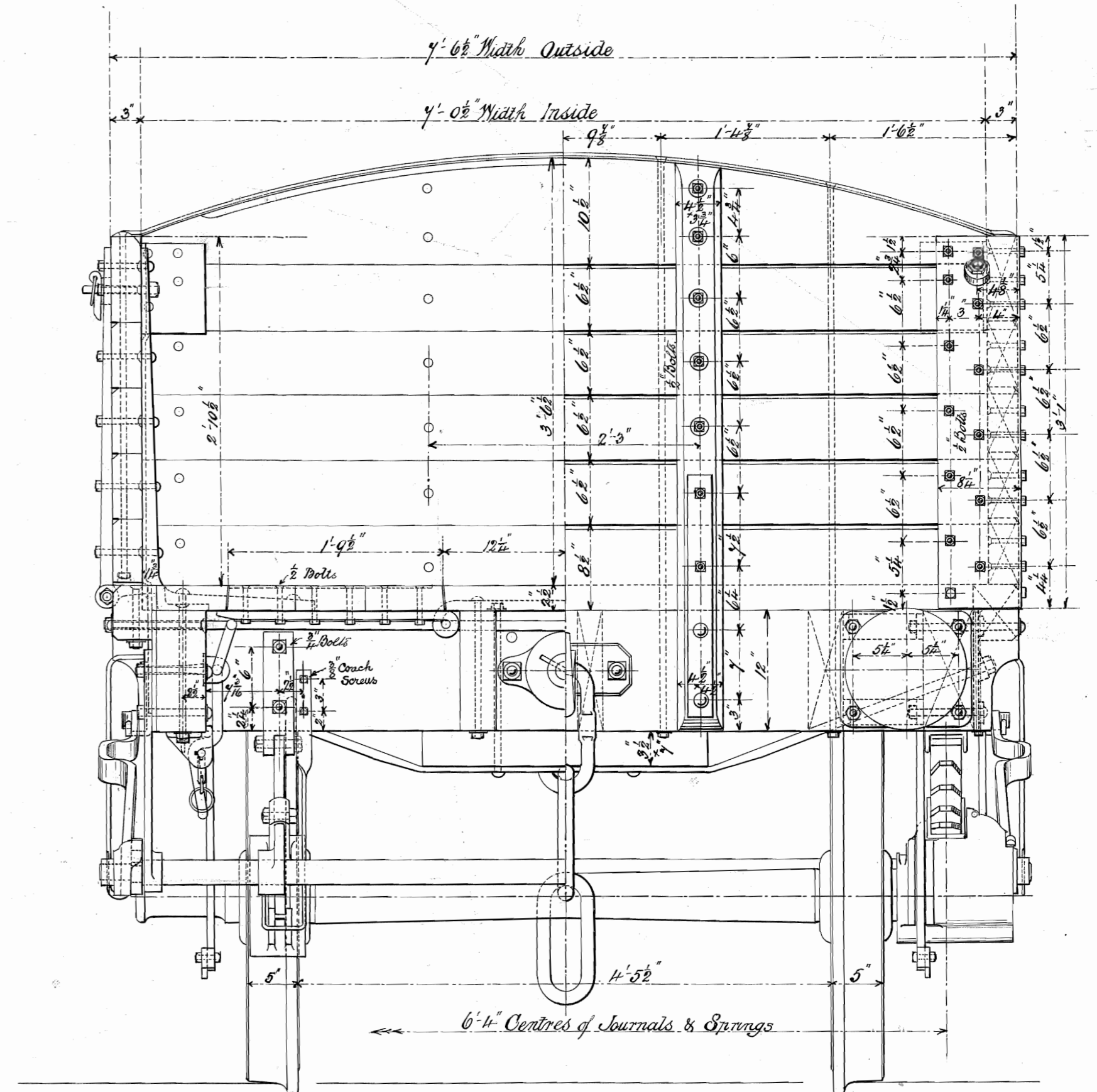
CROSS SECTION ON LINEAB HALF END ELEVATION
