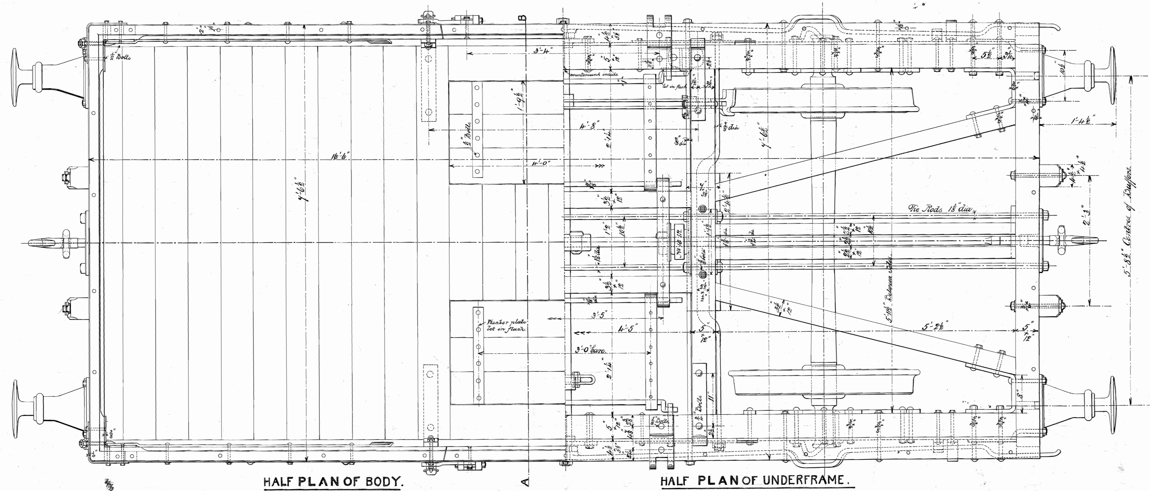
HALF PLAN OF BODY.
