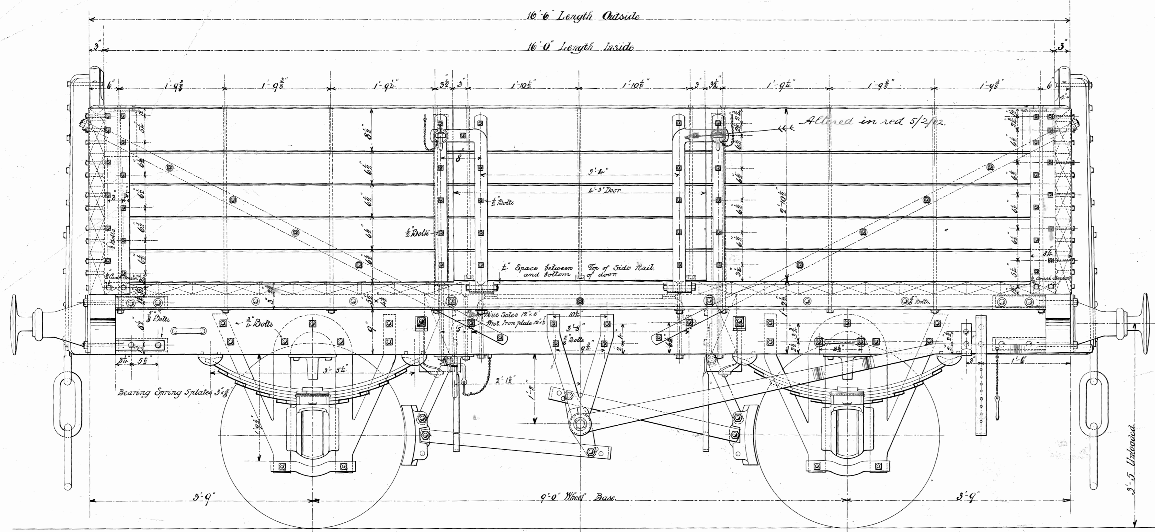
SIDE ELEVATION
