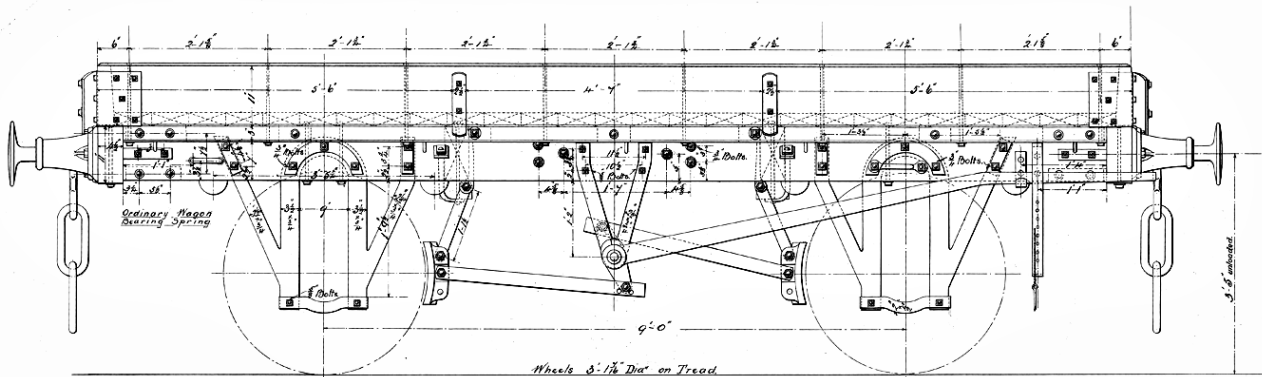
Wheels 5'-1 1/2" Dia on Tread Side Elevation.
