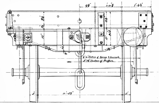
Half Cross Section of A.B. Half End Elevation.
