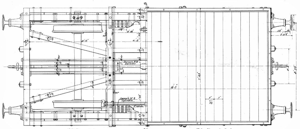
Half Plan of Underframe. Half Plan of Body.
