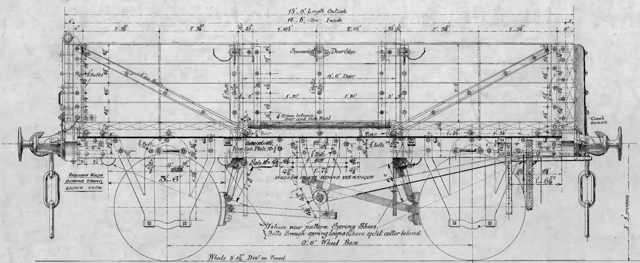
— SIDE ELEVATION —
