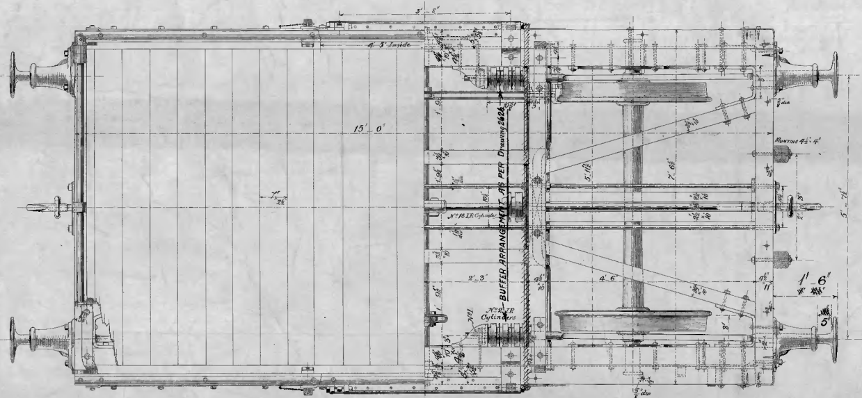
— HALF — HALF PLAN OF BODY — PLAN OF UNDERFRAME —
